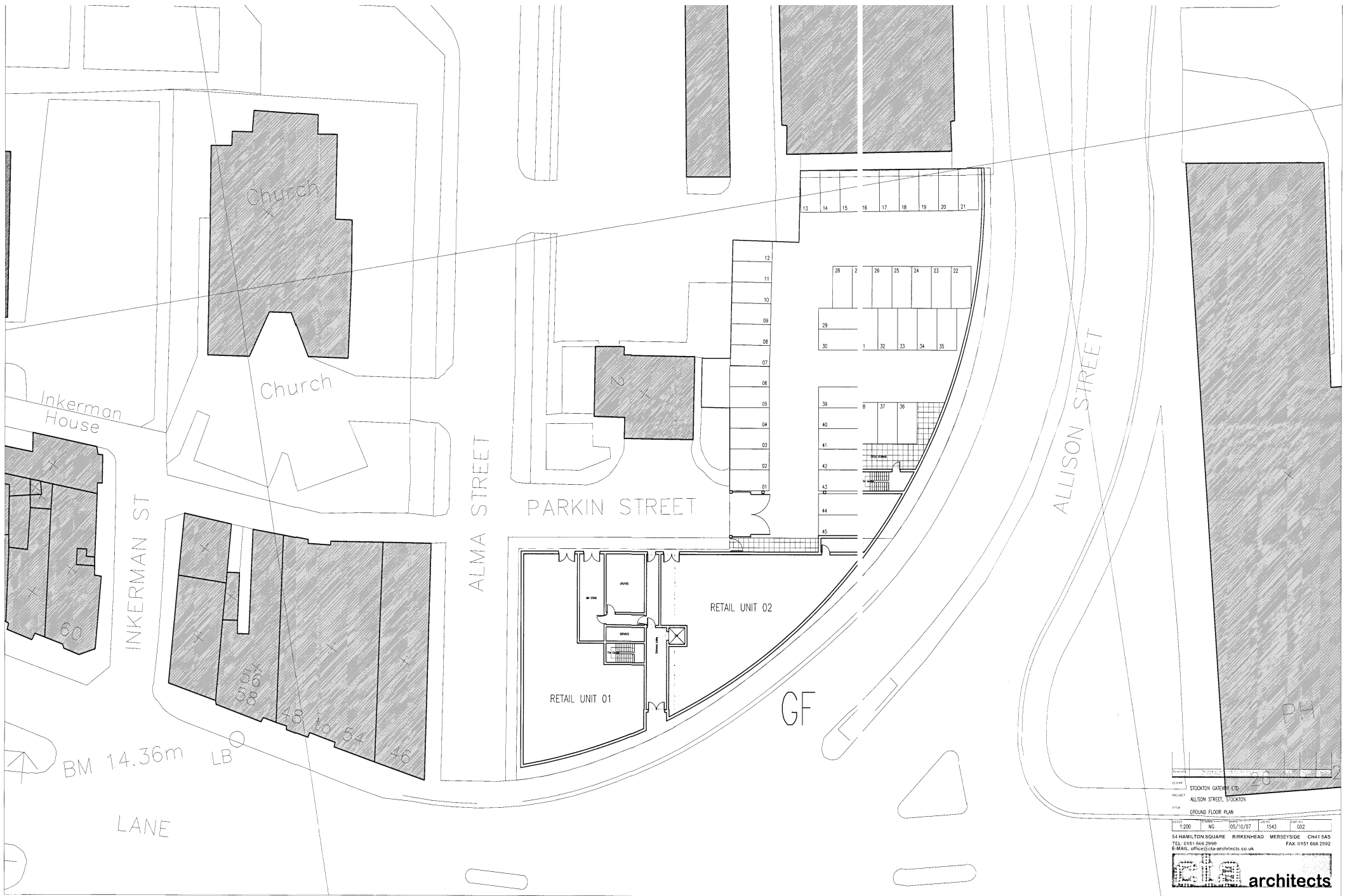
07/2893/OUT – Ground Floor Plan
